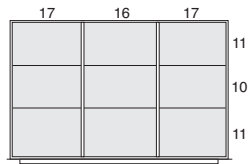
9 compartments NF0C ___ 4530
