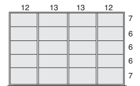
20 compartments NF0K ___ 4530
