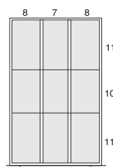
9 compartments NF0C 2230
