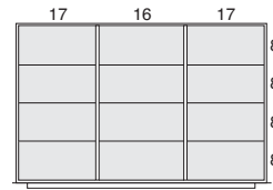
12 compartments NF0L ___ 4530
