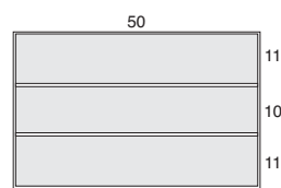
3 compartments NFAB _ _ _ 4530
