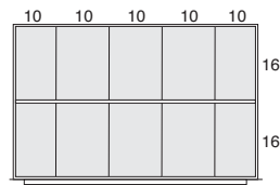
10 compartments NFAE ___ 4530
