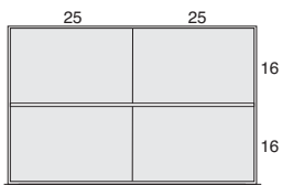
4 compartments NF0B _ _ _ 4530
