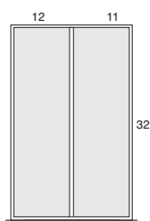
2 compartments NF0A 2230
