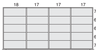
20 compartments NFOK ___ 6030
