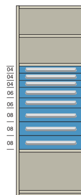
8 drawers, 5 shelves, (1) 36" support frame
