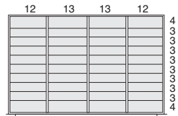
40 compartments NFMM ___ 4530
