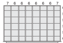
48 compartments NF0T ___ 4530
