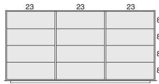
12 compartments NFOL ___ 6030
