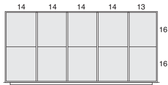
10 compartments NFAE ___ 6030
